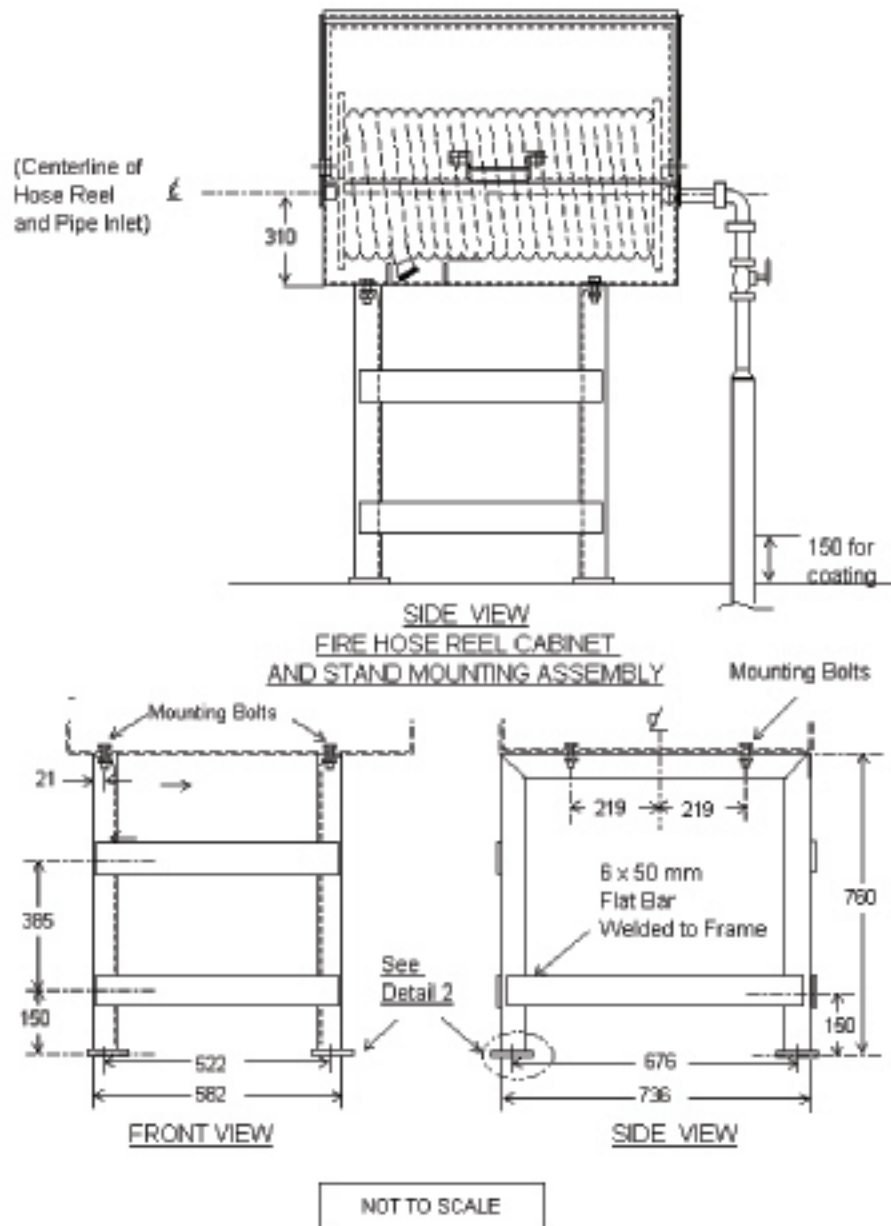
Figure 3 - Fire Hose Reel Cabinet
